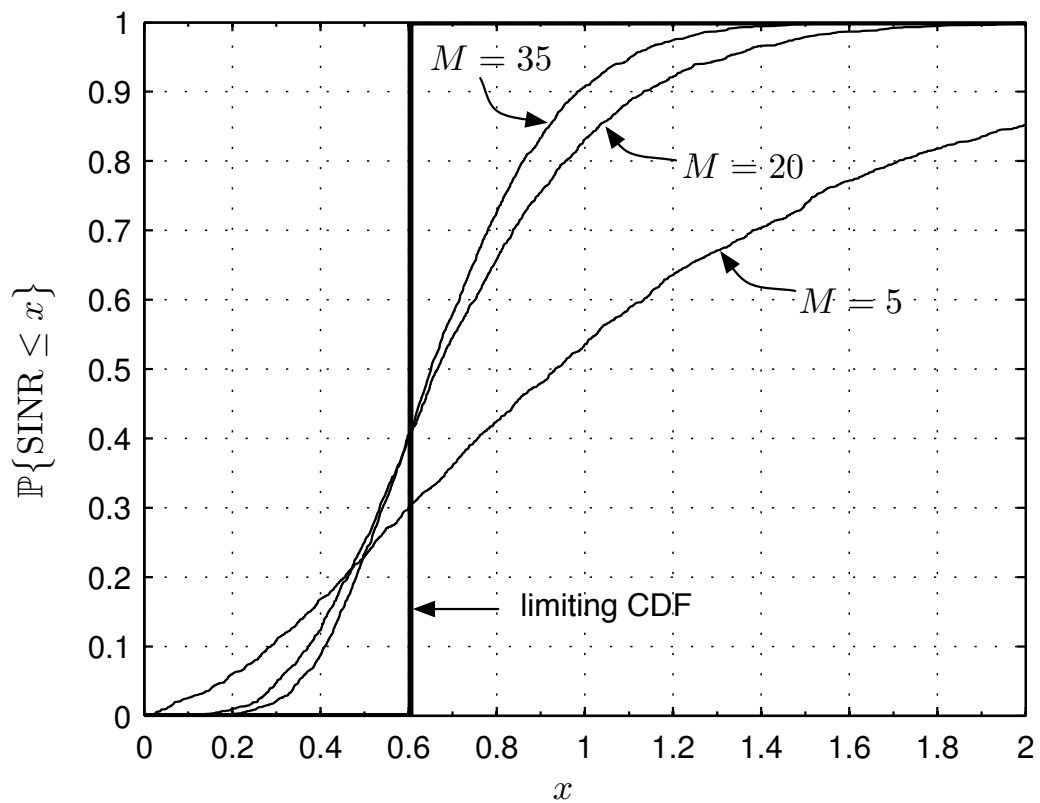
Fig. 3. Simulated (Monte-Carlo) SINR CDFs for different values of M for (a) K = M^3 in P1 and (b) K = M^2 in P2.
