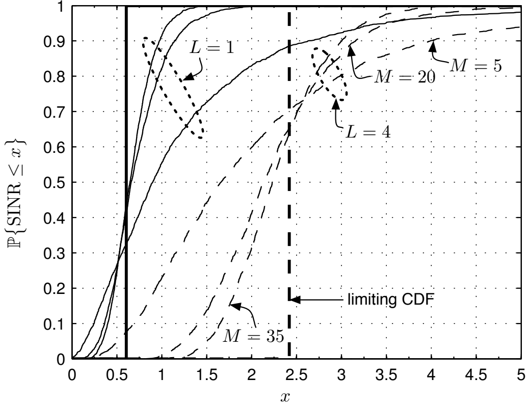
Fig. 4. Simulated (Monte-Carlo) SINR CDFs for different values of M for QL = M^3 in P1 with L = 4 .
