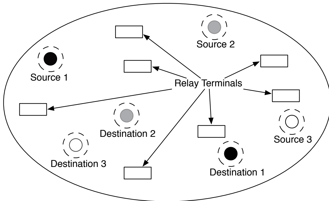
Fig. 1. Dense wireless network with dead-zones around source and destination terminals. Each terminal employs one antenna.
