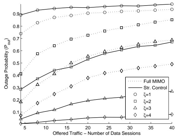
Fig. 2. Outage probability ( P_{out} ) of admitted QoS data sessions versus offered traffic for different values of the resource reservation margin \xi , with and without stream control ( N_0 = N_{max} = 6 ).
