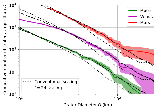
Figure 1 Crater populations on the Moon, Mars and Venus [after 2] (shading denotes uncertainty) compared with predictions based on the NEO population and crater scaling laws. To show on one plot, N(>D) has been scaled for Venus and Mars.
