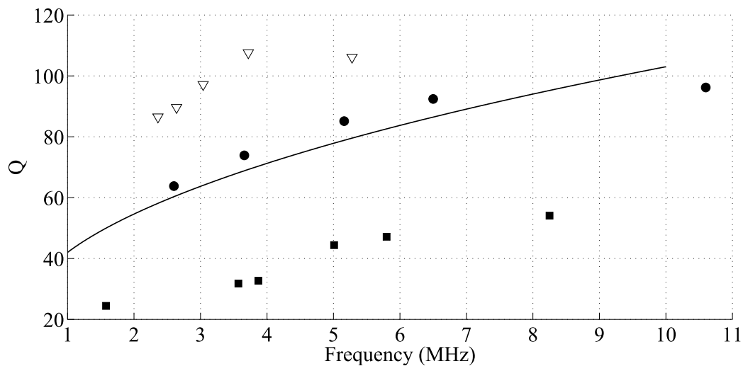
Figure 1. Q factor measurements and simulation results for 2cm coils. Simulation of solid wire coil —, Litz wire coil \nabla , Solid wire \bullet , PCB coil \blacksquare .
