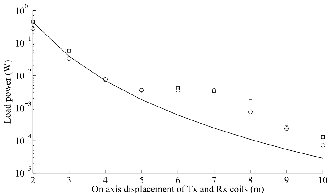
Figure 4. Load power transferred to 170 x 170mm Rx coil from 1 x1 m Tx coil with 98W DC power input to Tx amplifier. Simulation using round loops approximation —, Prediction using local magnetic field strength \square , Measured power at Rx coil \circ .
