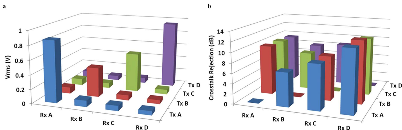
Figure 8 | Experiment for worst-case channel crosstalk. (a), Output RMS voltage for each receive (Rx) channel for different transmit (Tx) channels. (b), Calculated channel crosstalk rejection.
