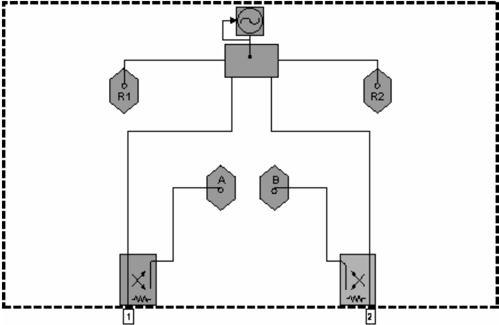
E8361A - Standard Configuration and Standard Power Range
