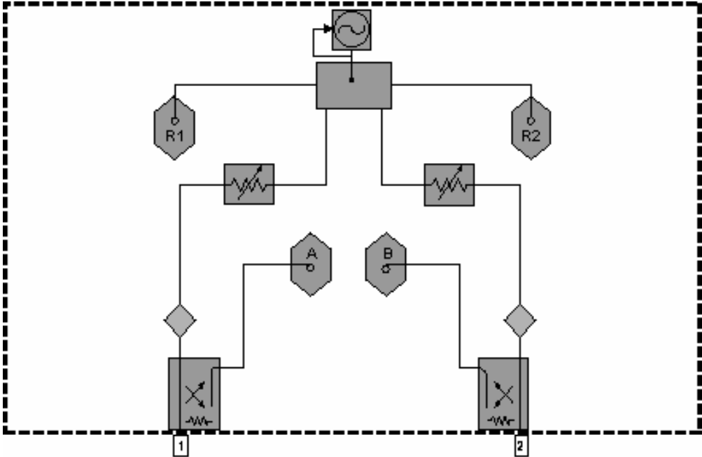
E8361A - Option UNL Standard Configuration with Extended Power Range and Bias - Tees
