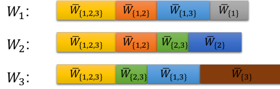
Fig. 1: An example of N = 3 correlated files. Each file consists of 4 different subfiles with different commonness levels.
