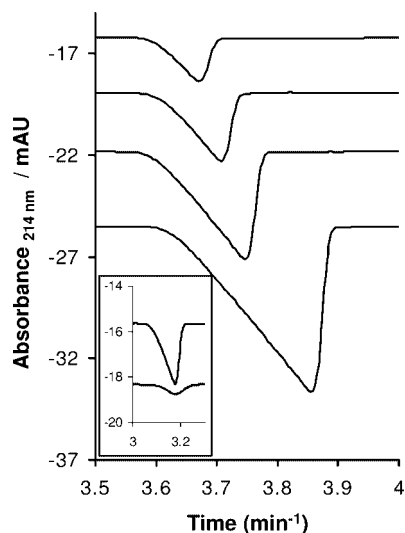
Figure 1. Traces for succinic acid calibration standards obtained using indirect-UV detection CE ( R^2 = 0.999 ; RSD = 3.48). Inset shows the CE traces for excess succinate in the triazine dendrimer reaction mixture after first and second purification cycles.
