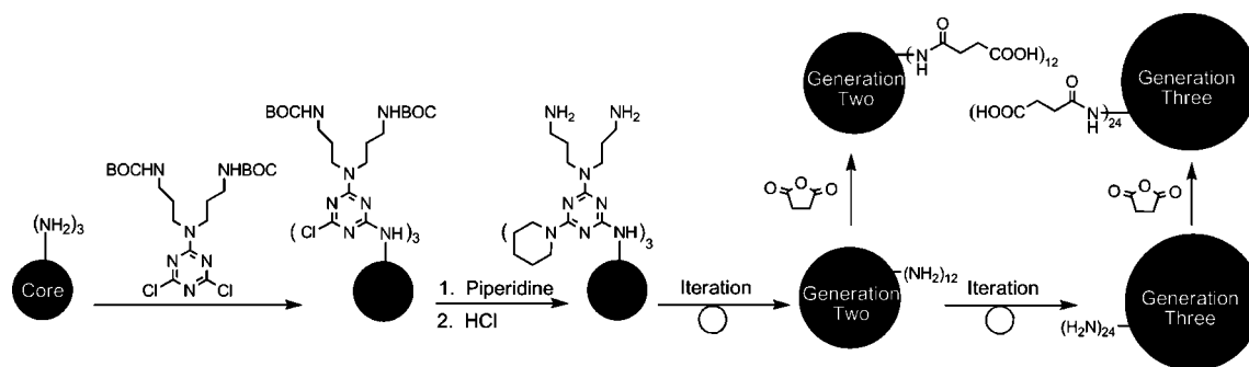
Scheme 1. Synthesis of the Anionic Triazine Dendrimers
