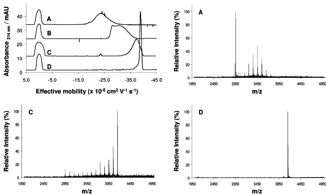
Figure 7. CE traces (top left) and corresponding MALDI-TOF-MS spectra for samples obtained during the monitoring of the succinylation of the second-generation triazine dendrimer: A = 0.25 mol succinic anhydride/mol \text{NH}_2 ; B = 0.5 mol succinic anhydride/mol \text{NH}_2 ; C = 0.75 mol succinic anhydride/mol \text{NH}_2 ; D = 1.0 mol succinic anhydride/mol \text{NH}_2 .
