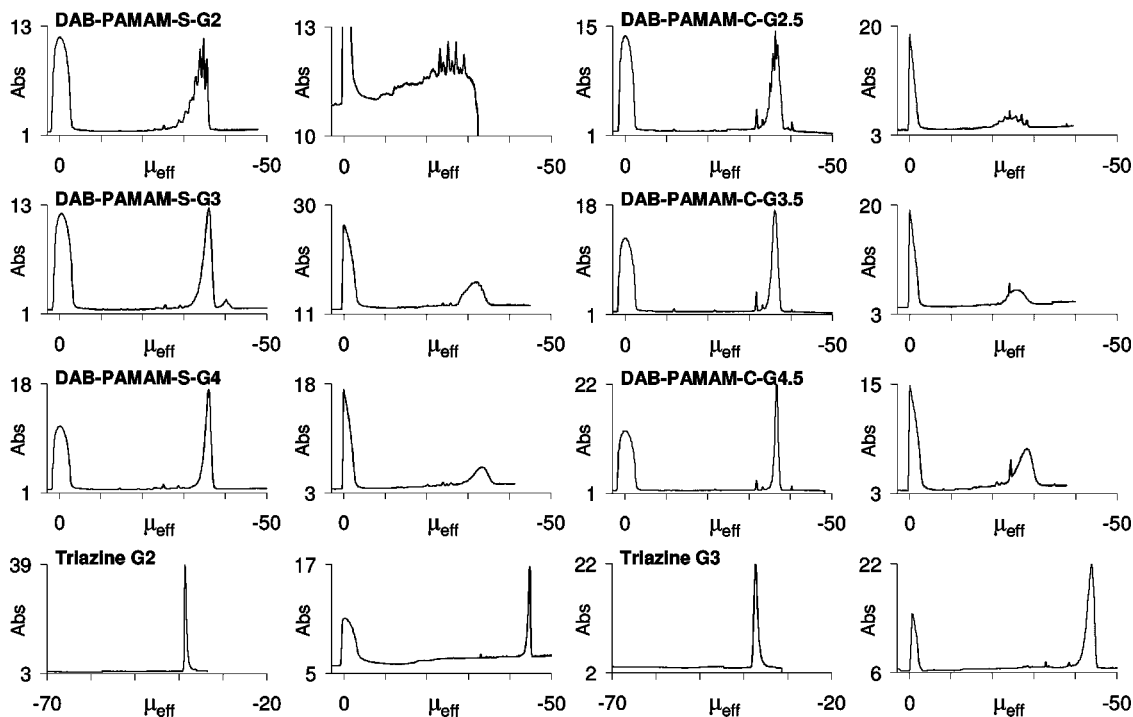
Figure 6. Electropherograms for the three dendrimer classes obtained using pH 9.1 100 mM borate/lithium buffer (left) and using pH 6.9 50 mM phosphate/lithium buffer (right). All traces were obtained in positive-to-negative polarity, except traces for triazine dendrimers using borate buffer, which were obtained in negative-to-positive polarity. The absorbance scale (Abs) is in milli-absorbance units (mAU) recorded at a 214 nm detection wavelength. Effective mobility scale ( \mu_{\text{eff}} ) is in " \times 10^{-5} \text{ cm}^2/\text{V}\cdot\text{s} " units.
